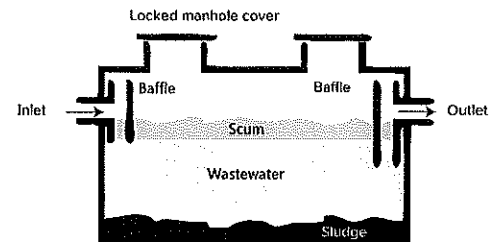
Typical Septic Tank
